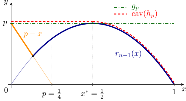
Figure 7: Concavification for n = 2 and p = 1/4 . The thick solid curve is h_p(x) = \max\{p-x, r_{n-1}(x)\} . The green dashed line is the affine function g_p used in the proof. The red dashed curve is the concave envelope of h_p(x) . At x = p , \text{cav}(h_p)(p) = g_p(p) = r_n(p) .
