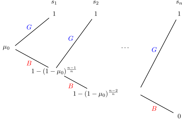
Figure 3: The asset's expected value in a Swiss cheese test.
