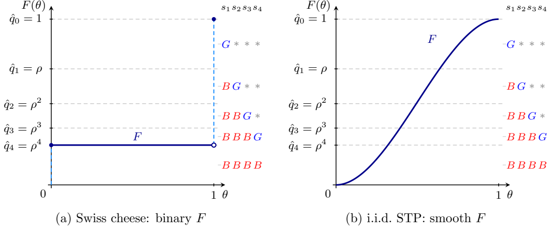
Figure 6: Examples of i.i.d. STP tests with four signals. Panel (a) depicts a Swiss-cheese test. Panel (b) depicts an i.i.d STP test with a smooth F . In both panels \rho = \Pr(s_i = B) denotes the probability of a B realization. The quantile thresholds are geometrically spaced because \hat{q}_i = \Pr(s_1 = \dots = s_i = B) = \rho^i .
