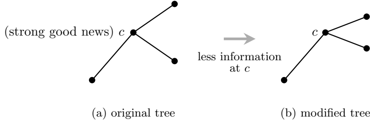
Figure 8: The first step. The height of each node represents its belief mean. Providing less information at a strong good news child c increases the option value at the parent of c more than it decreases the option value at c .
