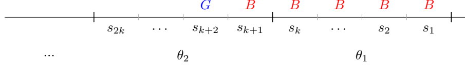
Figure 10: A possible realization of a layered Swiss-cheese test. The first G occurs at signal s_{k+2} , which is associated with \theta_2 . The asset value is therefore \theta_2 , regardless of subsequent signal realizations.
