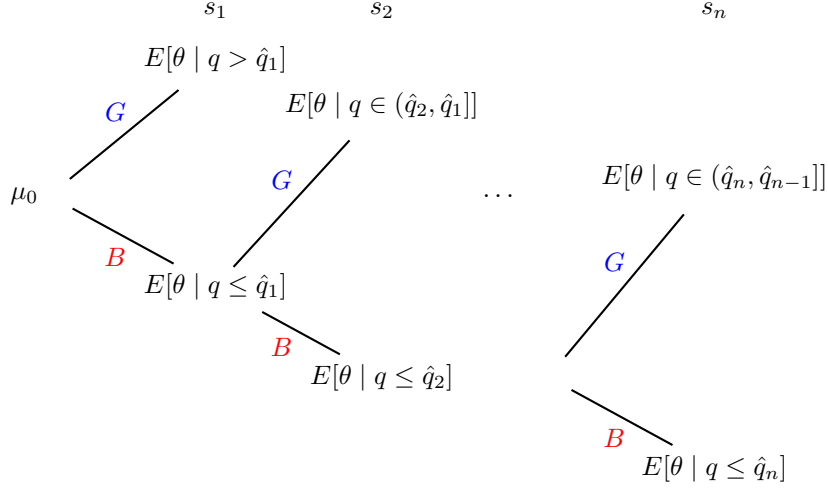
Figure 5: The asset's expected value in an STP test.
