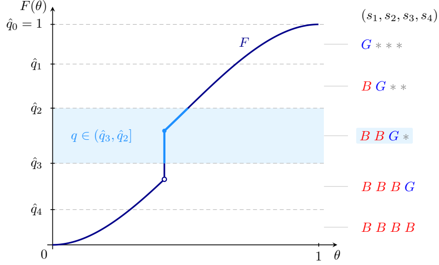
Figure 4: An STP test with four signals. If q \in (\hat{q}_i, \hat{q}_{i-1}] , the first G occurs at signal i : s_1 = \dots = s_{i-1} = B and s_i = G . The shaded band illustrates q \in (\hat{q}_3, \hat{q}_2] , which corresponds to the realization (B, B, G, *) , where * denotes either G or B . If q \leq \hat{q}_4 , all signal realizations are B .
