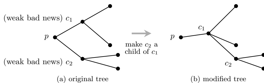
Figure 9: The third step. The height of each node represents its belief mean. Making c_2 a child of c_1 increases the option value of c_1 without affecting the option value elsewhere.
